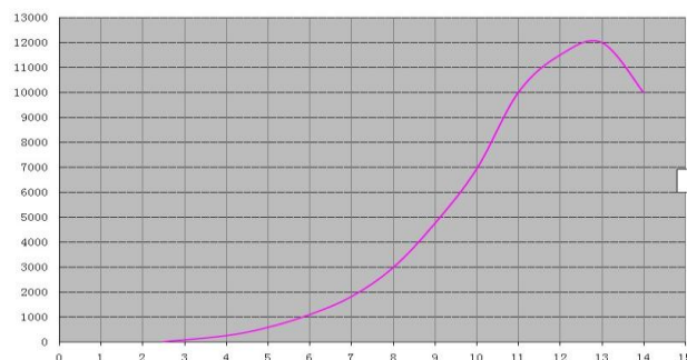
EN-10KW-G wind turbine power curve
