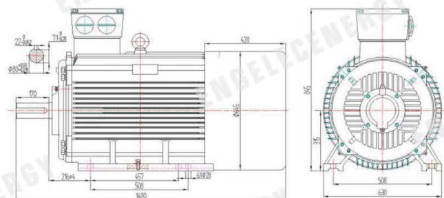
EN-140KW-450R-60Hz-120V Drawing
