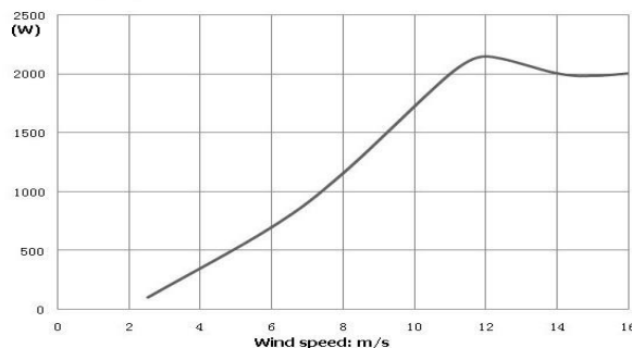
EN-2KW-L wind turbine power curve
