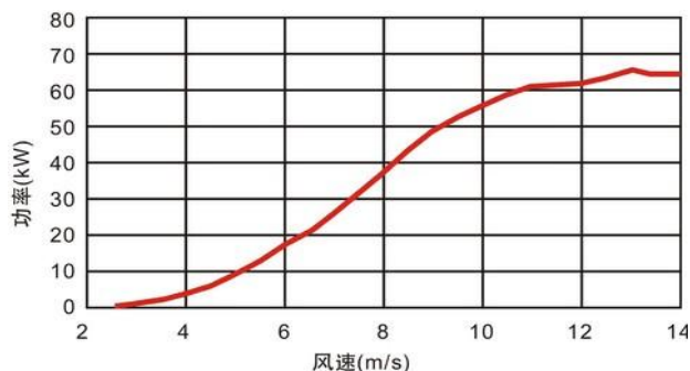
EN-50KW-E wind turbine power curve
