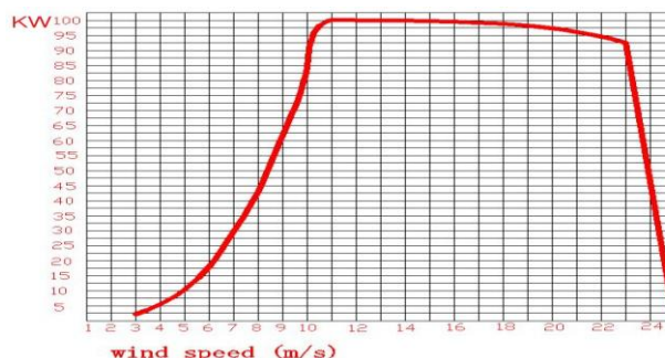
EN-100KW-E wind turbine power curve
