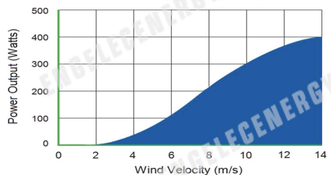
EN-400W-XL Wind Turbine Power Curve
