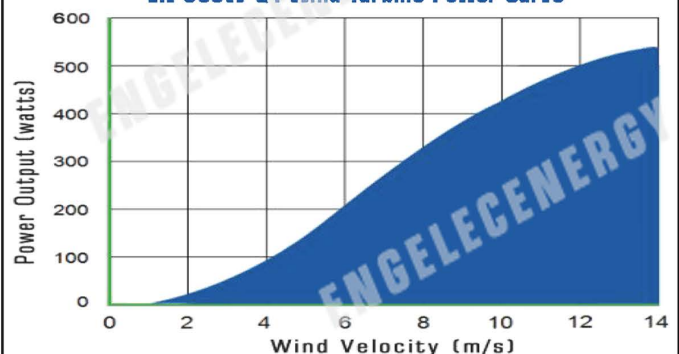
EN-500W-Q4 Wind Turbine Power Curve
