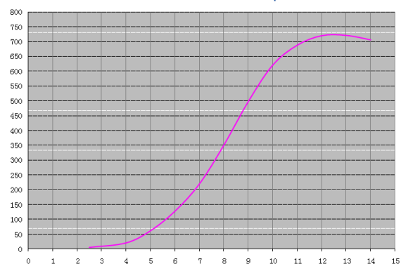
EN-700W-M4 wind turbine power curve
