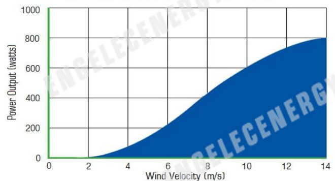
EN-800W-XL Wind Turbine Power Curve
